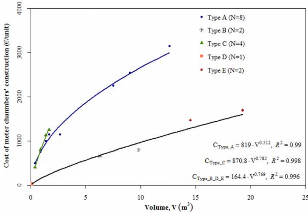
Figure 4 | Construction cost of meter chambers as a function of the volume in WSS.
