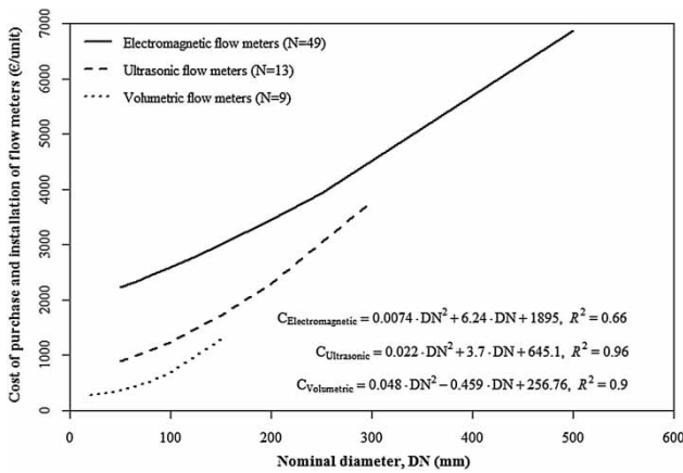
Figure 5 | Purchase and installation cost of flow meters as a function of nominal diameter in WSS.
